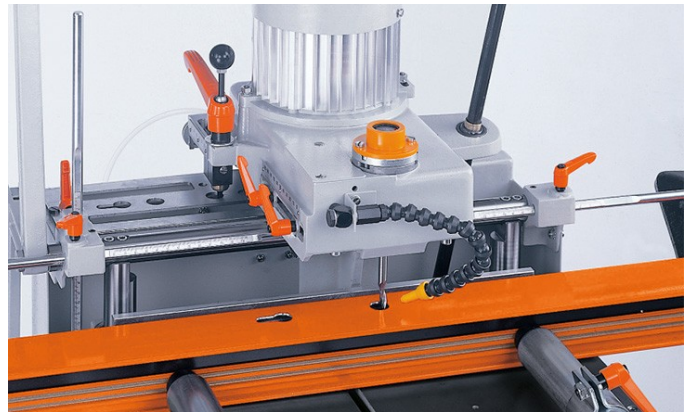
1-spindle copy router AS 70/44
